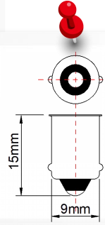
BA9S Base
