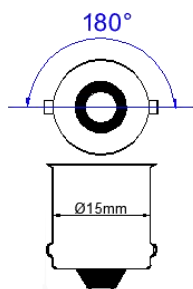
BA15S-(R10W)
