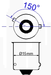
BAU15S-(RY10W)
